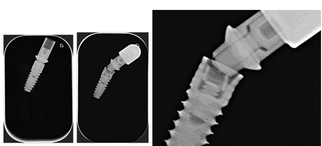
FIGURE 8. Group II: radiograph evaluation of the internal hexagon joint implant tested. Left: Prior fracture strength test. Middle: after the loading. Right: detail of the implant-joint connection after the test.
